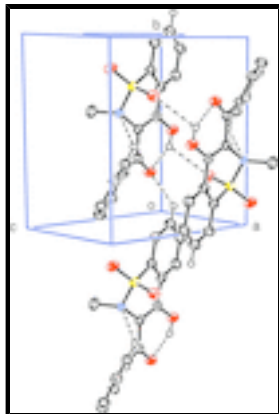
Fig. 2. A part of the unit cell showing intermolecular and intramolecular hydrogen bonds by dashed lines; the H-atoms not involved in H-bonds have been excluded for clarity.
