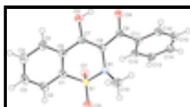
Fig. 1. The title molecule plotted with the displacement ellipsoids at 50% probability level (Farrugia, 1997).
